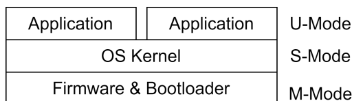
Figure 1: RISC-V Privilege Levels
